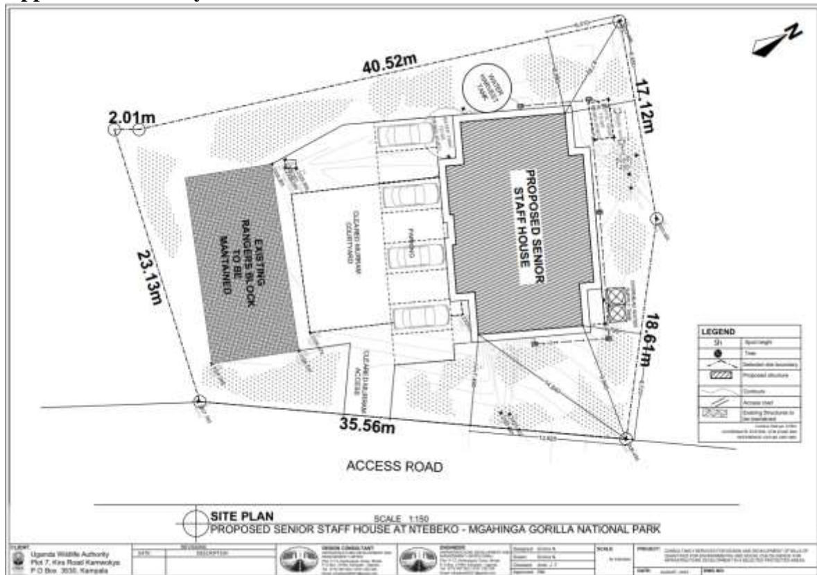
Figure 16: Ntebeko Senior Staff Accommodation Site Plan
