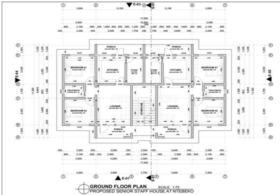
Figure 6: Senior Staff Houses Floor Plan Design
