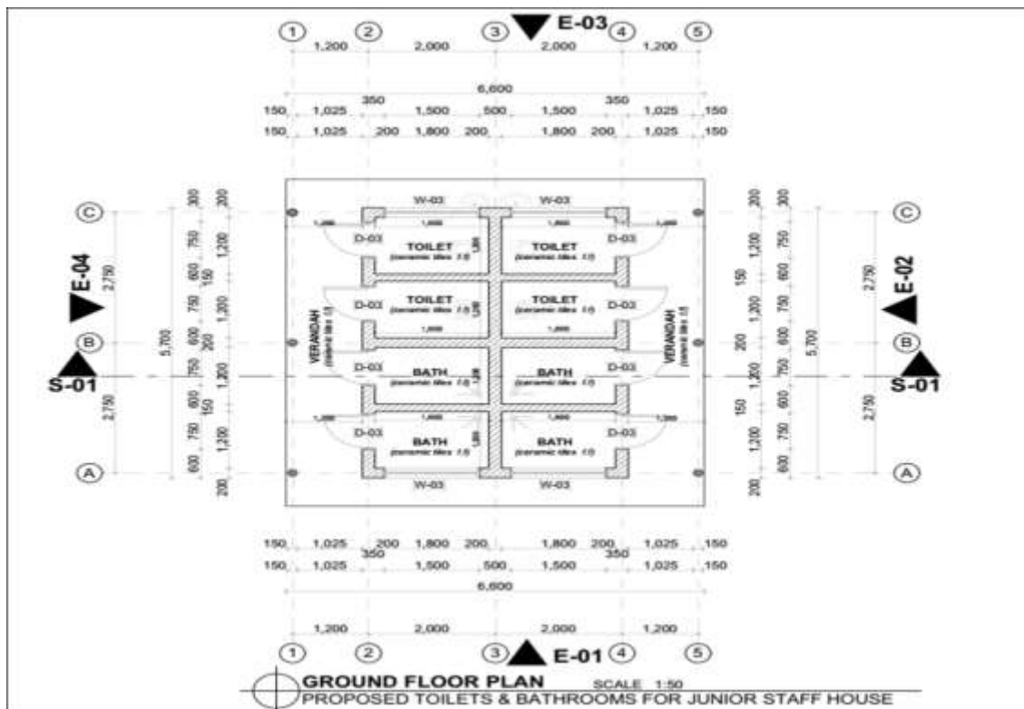
Figure 10: Ablution Block -Floor Plan Design
