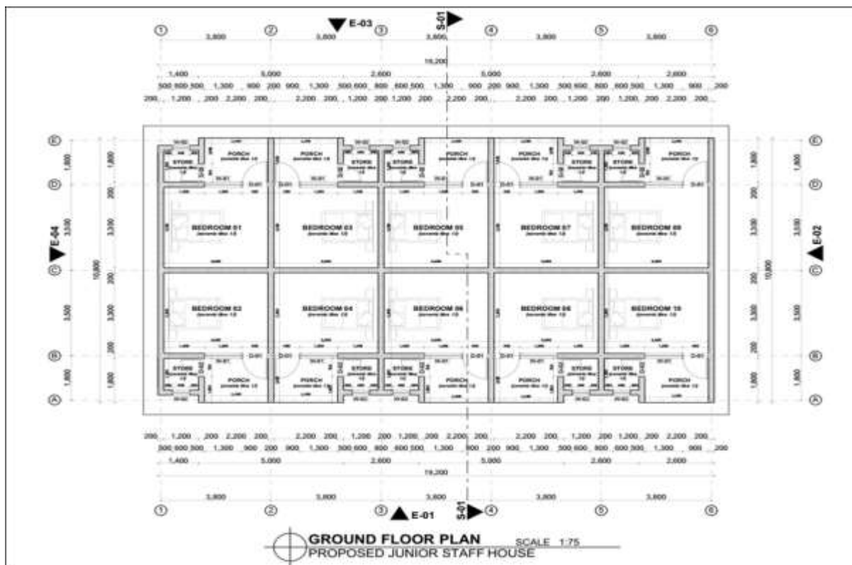
Figure 4: Junior Staff Houses Floor Plan Design
