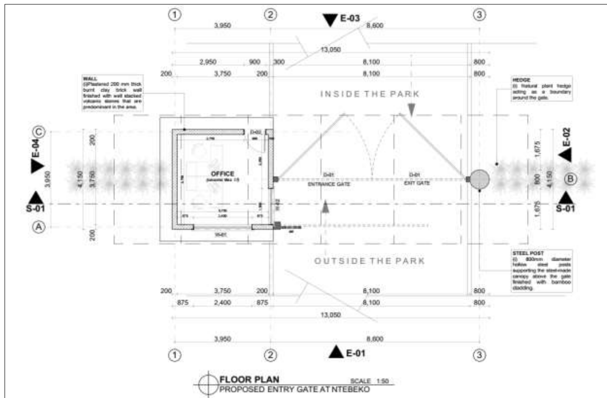
Figure 12: Mgahinga Gorilla National Park Ntebeko Gate Floor Plan
