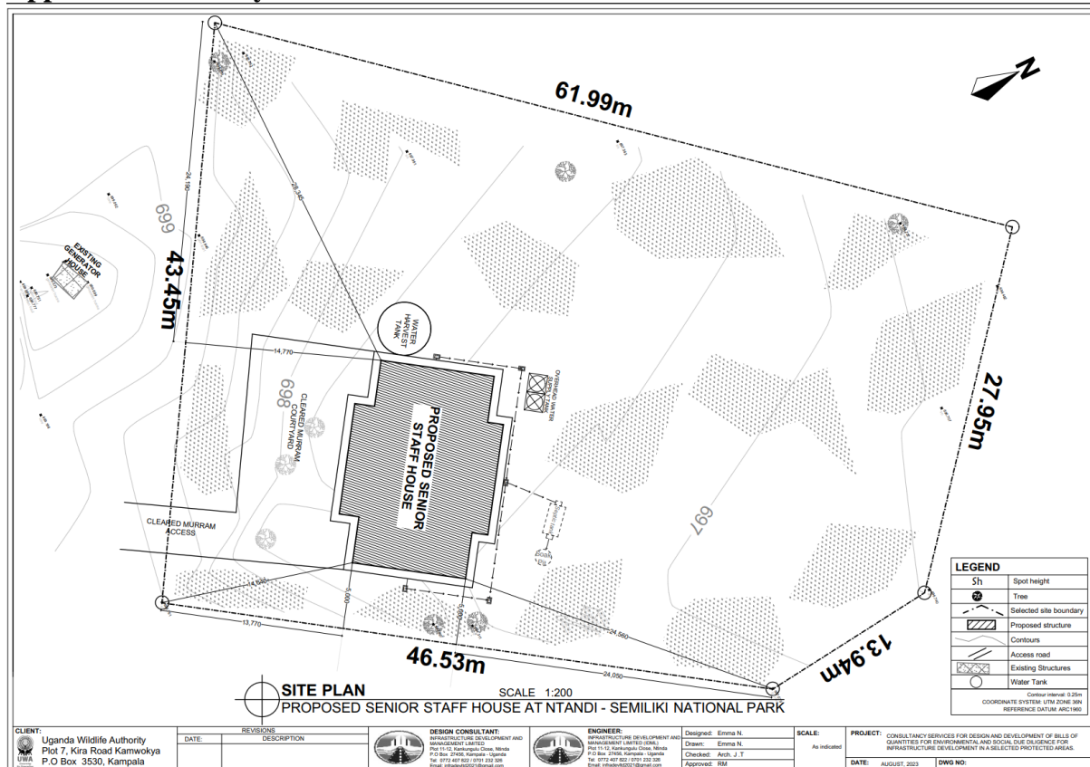
Figure 19: Ntandi Senior Staff Accommodation Site Plan
