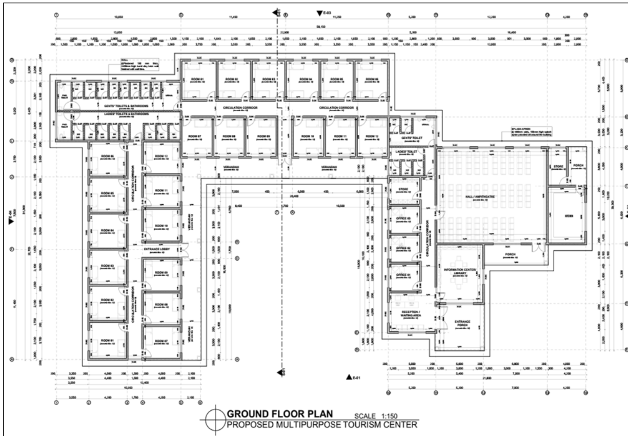
Figure 14: Semliki National Park Sempaya Tourism Centre Floor Plan
