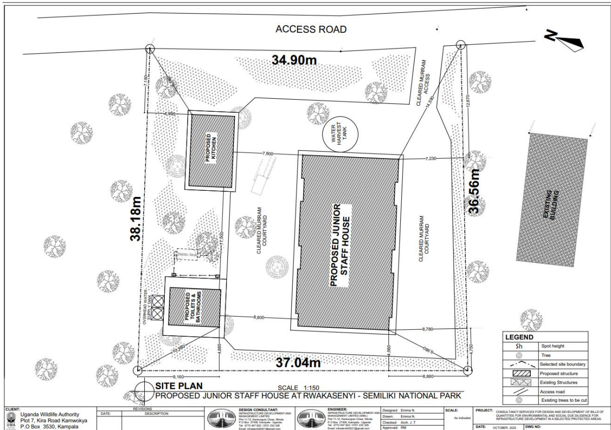
Figure 21: Rwakasenyi Junior Staff Accommodation Site Plan
