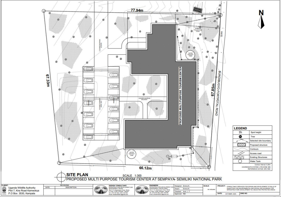
Figure 23: Sempaya Tourism Center Site Plan
