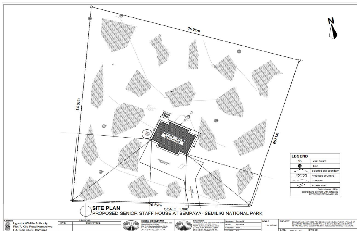
Figure 20: Sempaya Senior Staff Accommodation Site Plan
