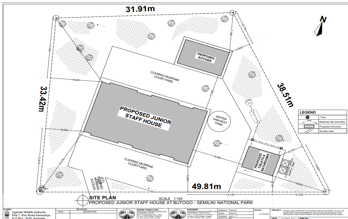
Figure 22: Butogo Junior Staff Accommodation Site Plan
